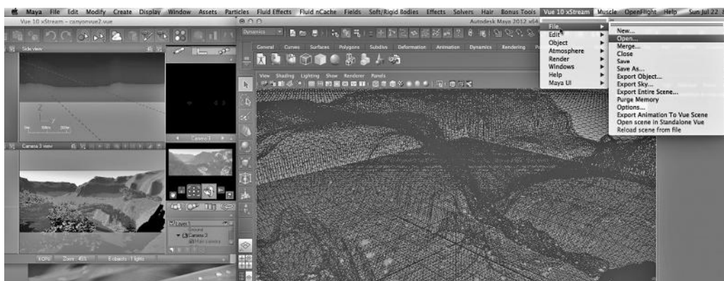
FIGURE 14.3 Vue plug-ins.
