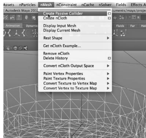
FIGURE 6.11 Passive collider.
