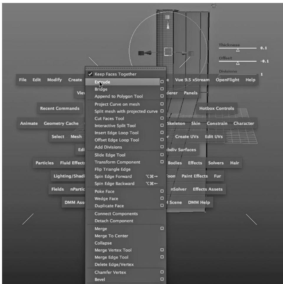
FIGURE 4.45 Extrude tool.
