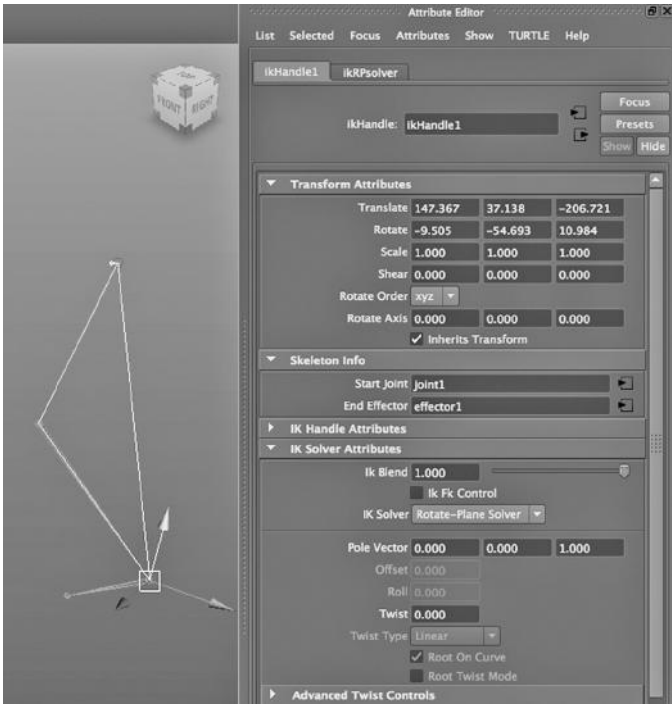
FIGURE 11.12 The Rotate Plane solver.
