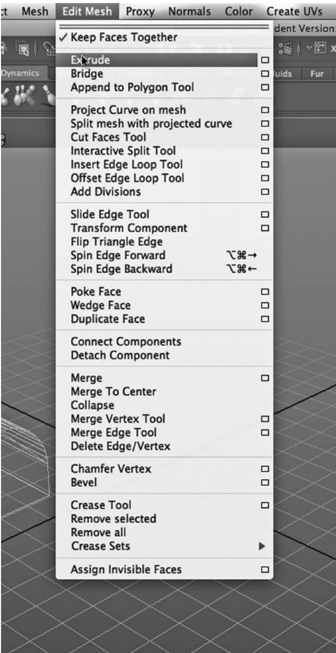
FIGURE 4.18 Extrude tool.
