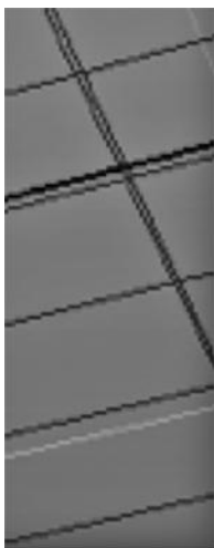
FIGURE 4.92 Before merging.
